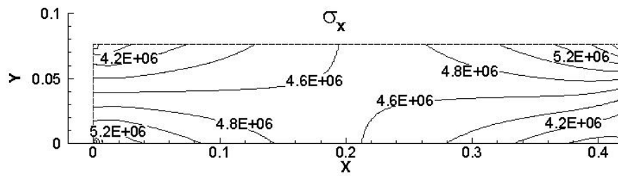
Figure 13 Longitudinal stress for test # 2 (Pa)
