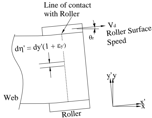
Figure 7 Coordinate transformation for normal strain
